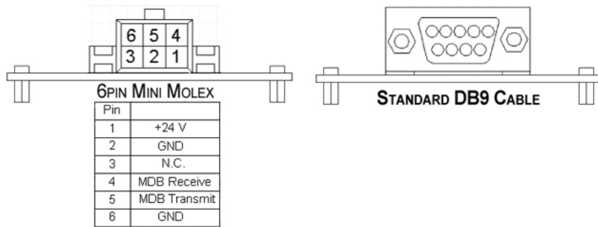
Figure-2 Connector Pin Outs
