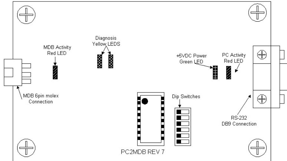
Figure 1 - Connector, Jumper, and LED locations
